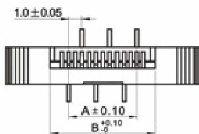
正针排列 Positive-needle arrangement
