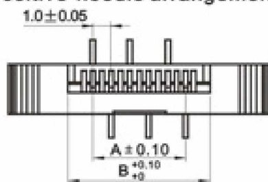
反针排列 Negative-needle arrangement
